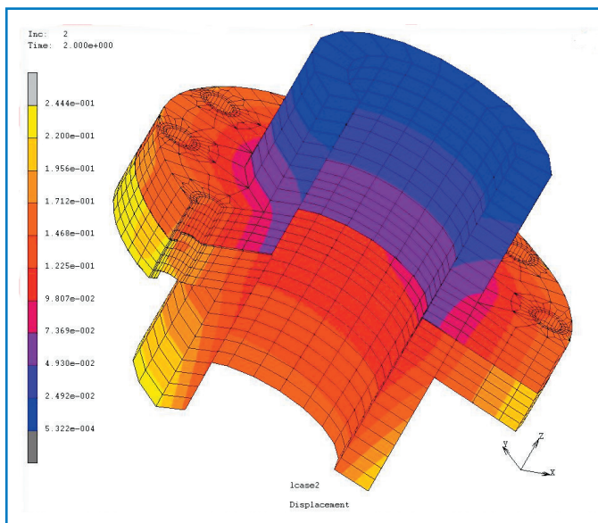
Finite element analysis with installed Expansion Bolts (100 x Enlargement)
