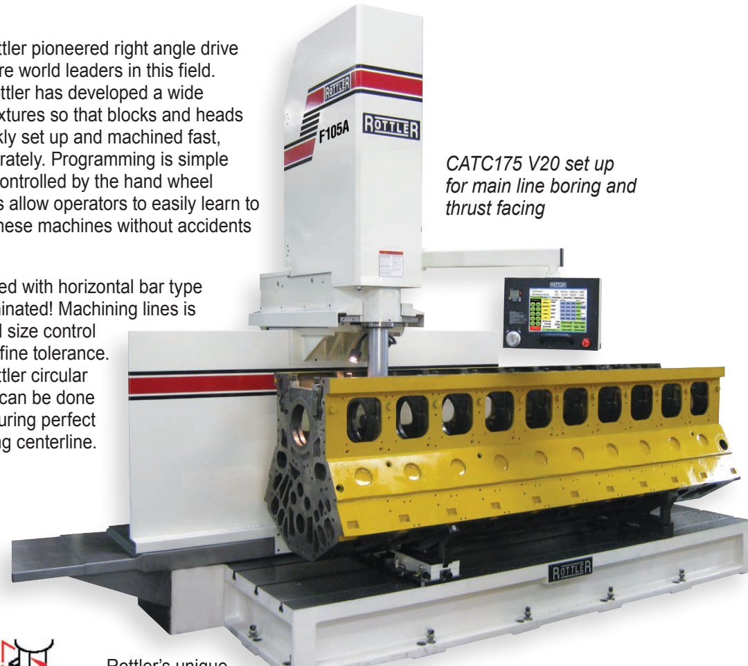
Rottler's unique right angle drives machine each bore individually and the digital display ensures perfect accuracy and alignment.
