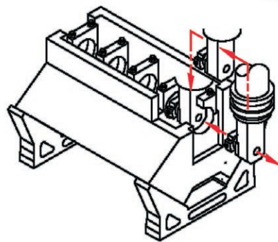
Rottler's unique right angle drives machine each bore individually and the digital display ensures perfect accuracy and alignment.
